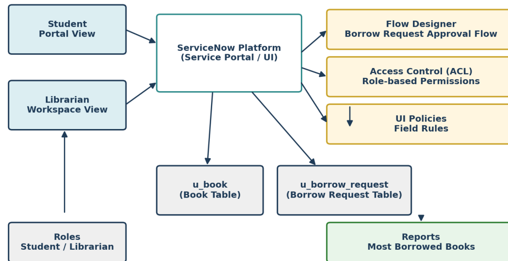
Figure 1: Library Management System - Solution Architecture (ServiceNow)
